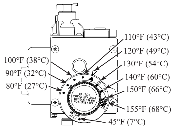
Temperature Dial
